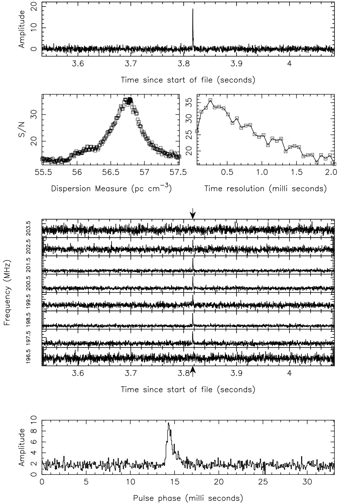
FIG. 1.—Bright giant pulse detected with the MWA-LFD early deployment system. Top: Dedispersed time series of a short data segment near the giant pulse. Middle panels: Diagnostic plots from the giant pulse search processing; plots of S/N vs. dispersion measure and time resolution, and dedispersed time series for eight subbands, each 1 MHz wide, within the 8 MHz bandwidth. Bottom: The dedispersed pulse shown in high time resolution. The scattering tail is clearly visible.
